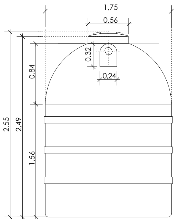
VISTA FRONTAL
